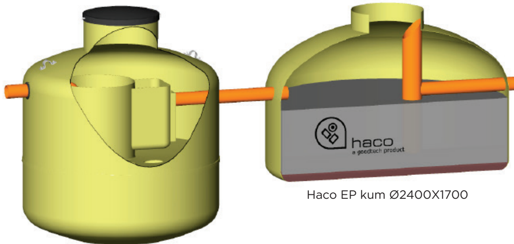
Slamavskiller BG 2 m 3
